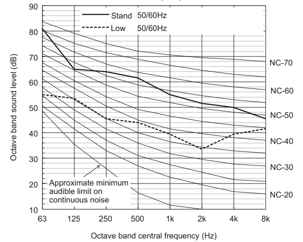
Sound level of PURY-P450YSNW-A(-BS)
