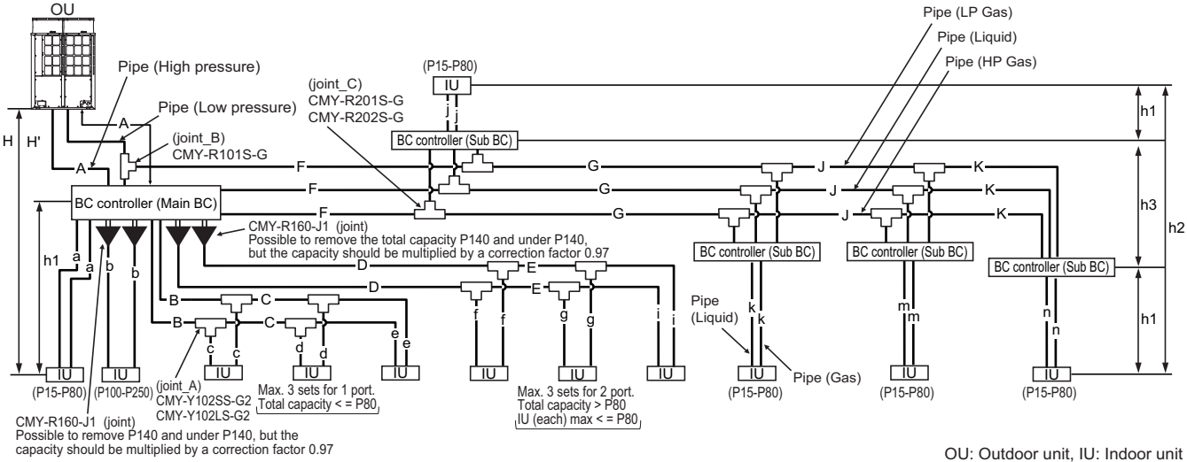
Fig. 12-2-2A Piping scheme
