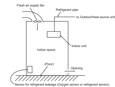
Fig. 1-3. Fresh air supply upon sensor action
