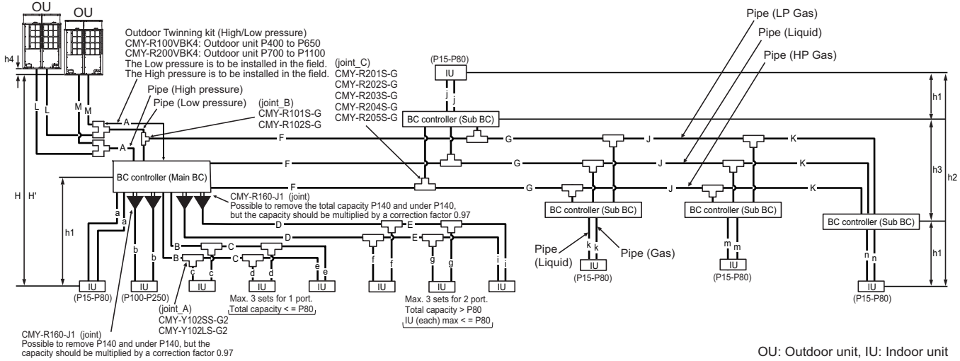
Fig. 12-2-3A Piping scheme
