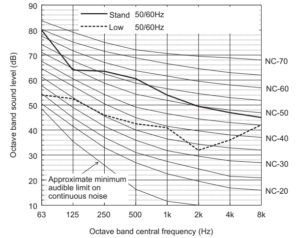
Sound level of PURY-P400YSNW-A(-BS)
