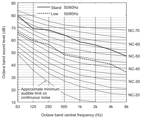
Sound level of PURY-P550YNW-A(-BS)
