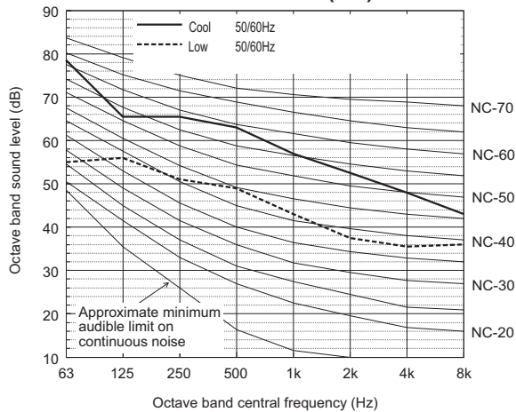
Sound level of PUHY-P600YSNW-A1(-BS)
