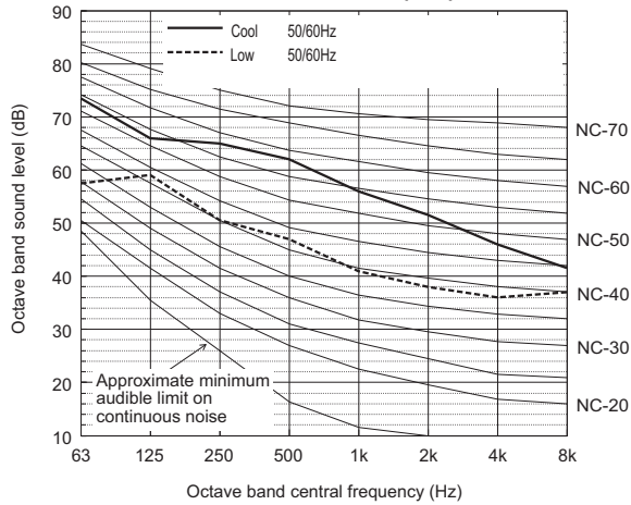
Sound level of PUHY-P500YSNW-A1(-BS)
