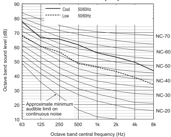
Sound level of PUHY-P500YNW-A1(-BS)
