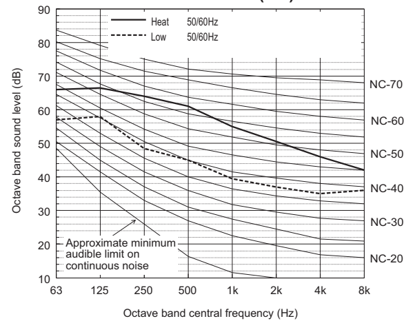
Sound level of PUHY-P400YSNW-A1(-BS)
