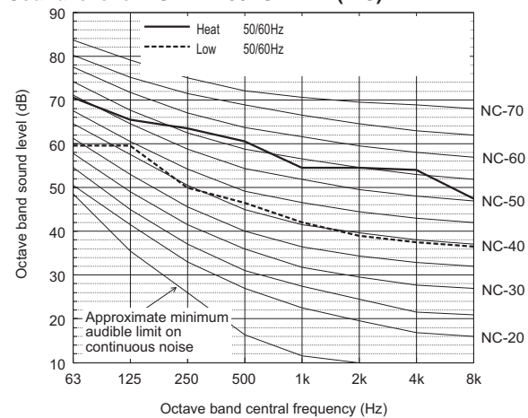
Sound level of PUHY-P450YSNW-A1(-BS)
