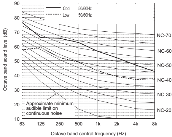
Sound level of PUHY-P550YSNW-A1(-BS)
