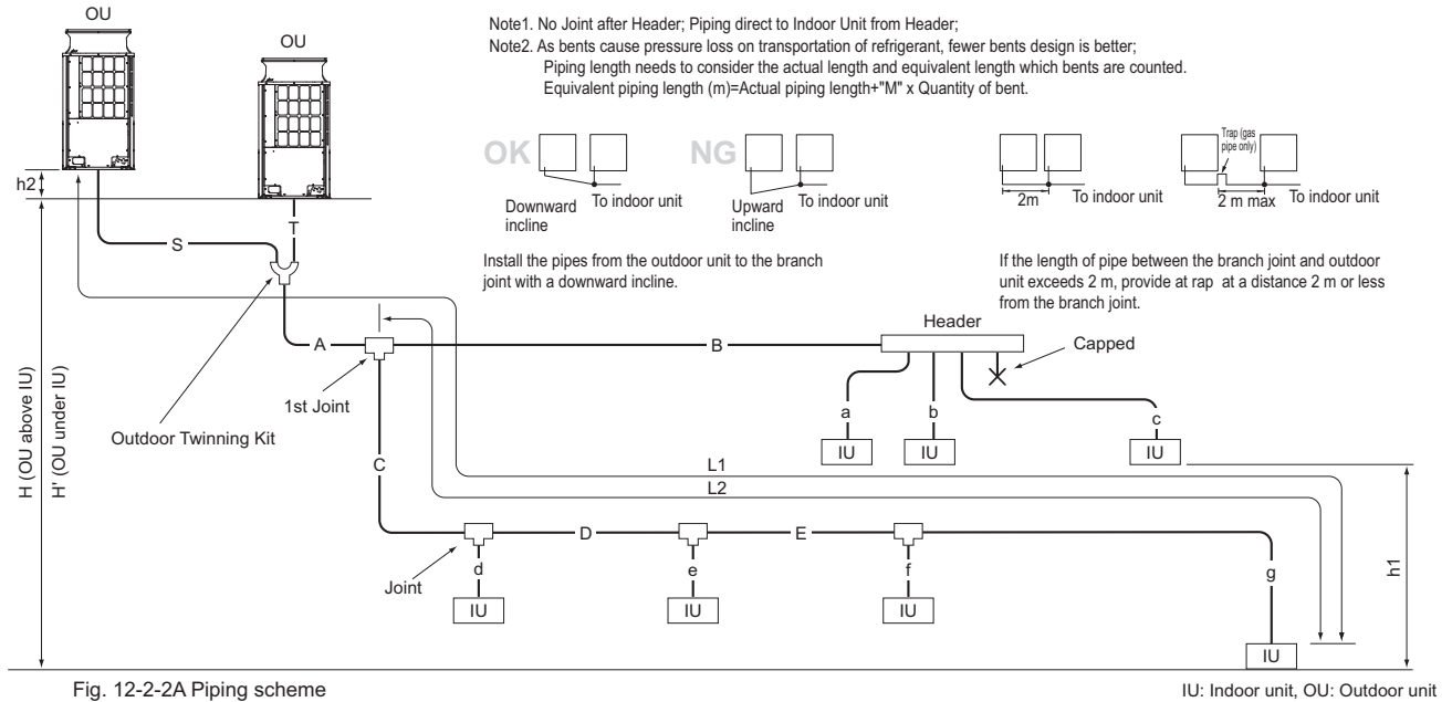
Fig. 12-2-2A Piping scheme
