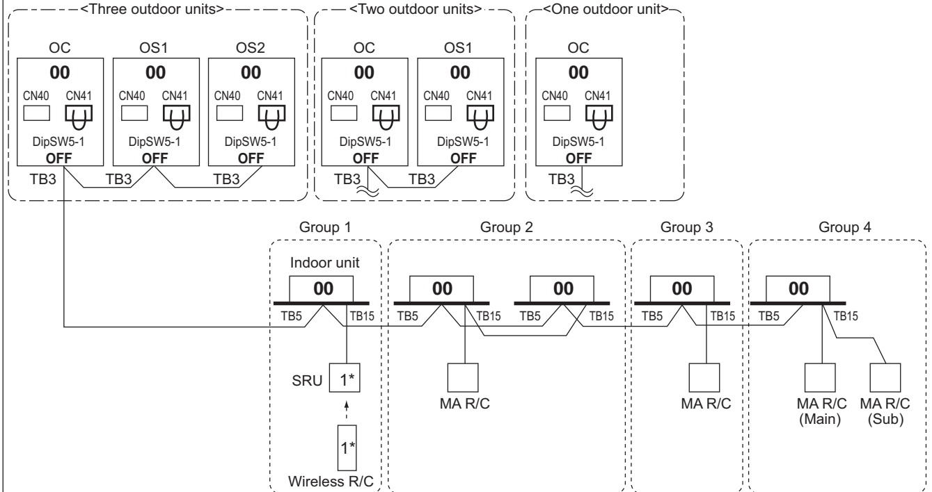
11-4-3-1. MA remote controller, Single-refrigerant-system, No System Controller
