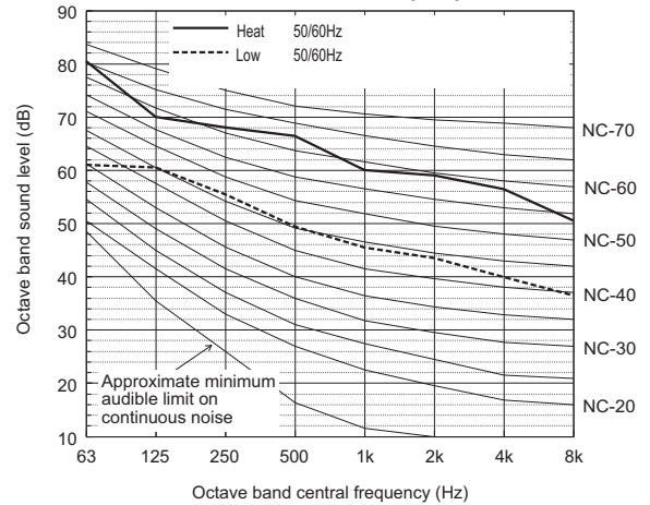
Sound level of PUHY-P650YSNW-A1(-BS)
