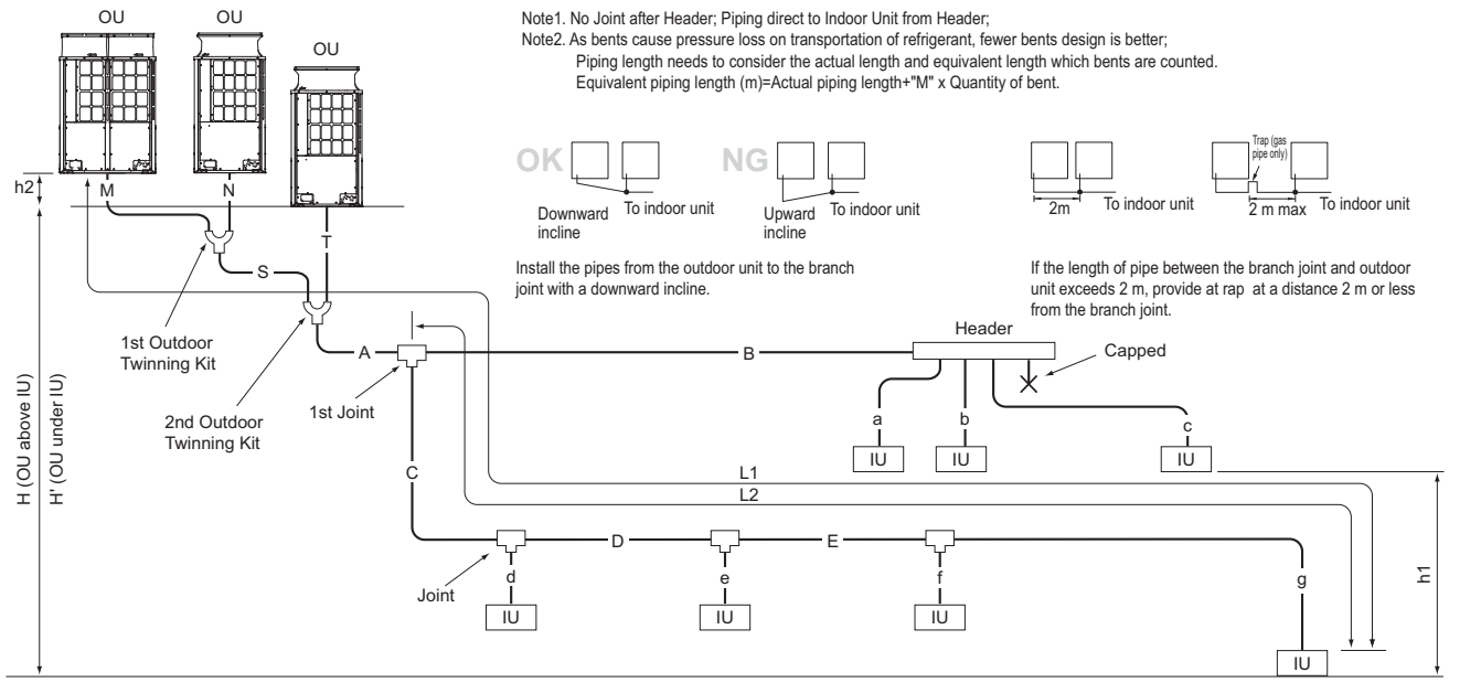
Fig. 12-2-3A Piping scheme
